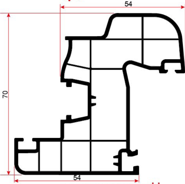
7025 PERVAZLI KASA PROFİLİ FRAME PROFILE WITH SILL
