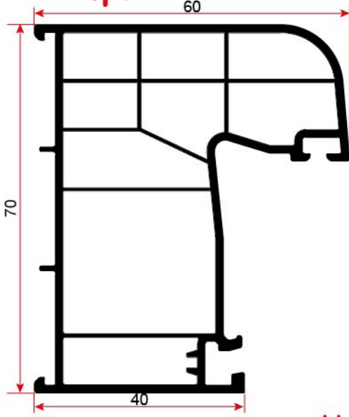
7003 DAMLALIKLI KANAT PROFİLİ DRAINED SASH PROFILE
