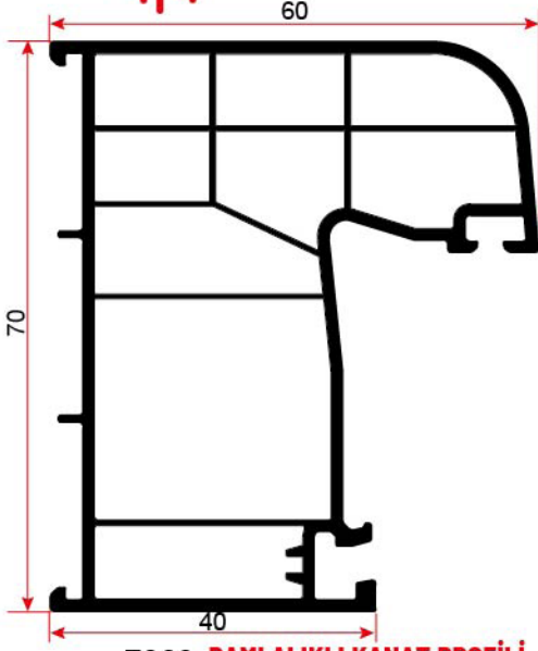
7023 DAMLALIKLI KANAT PROFİLİ DRAINED SASH PROFILE
