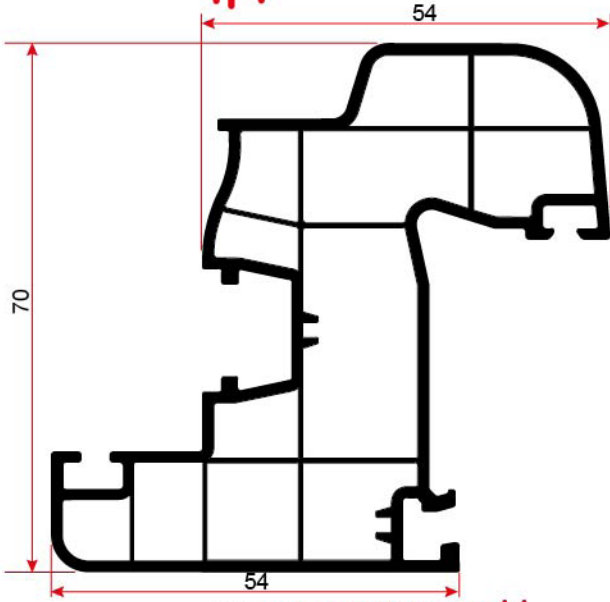
7005 PERVAZLI KASA PROFİLİ FRAME PROFILE WITH SILL
