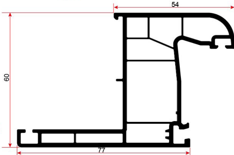
6005 PERVAZLI KASA PROFİLİ FRAME PROFILE WITH SILL
