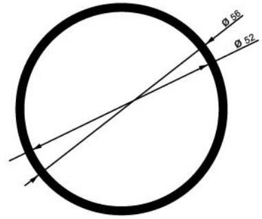
9003 BORU PROFİLİ PIPE PROFILE
