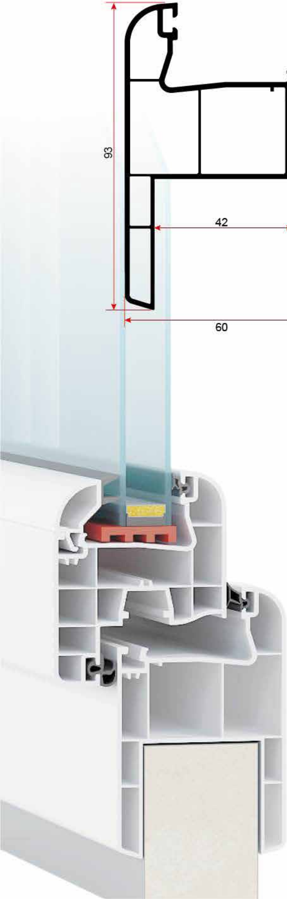
3001 40'LİK U KASA PROFİLİ 40' U FRAME PROFILE
