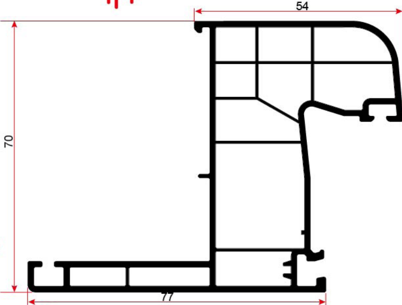
7025 PERVAZLI KASA PROFİLİ FRAME PROFILE WITH SILL
