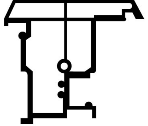
9003 BORU PROFİLİ PIPE PROFILE
