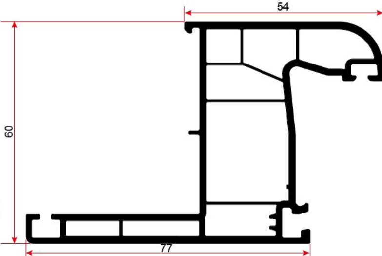
6025 PERVAZLI KASA PROFİLİ FRAME PROFILE WITH SILL
