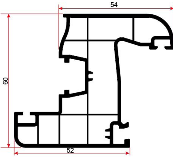
6025 PERVAZLI KASA PROFİLİ FRAME PROFILE WITH SILL
