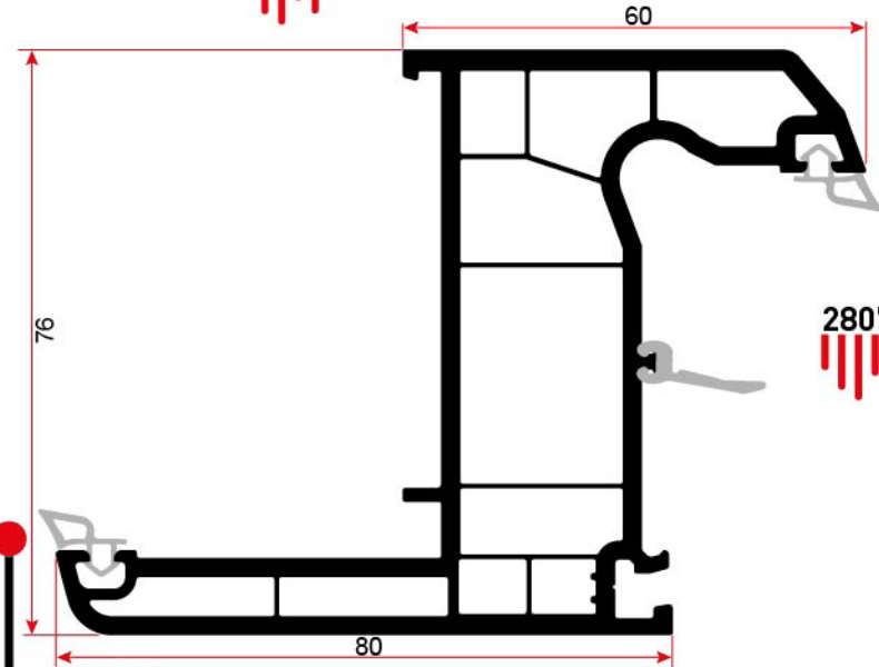
2205 PERVAZLI KASA PROFİLİ FRAME PROFILE WITH SILL
