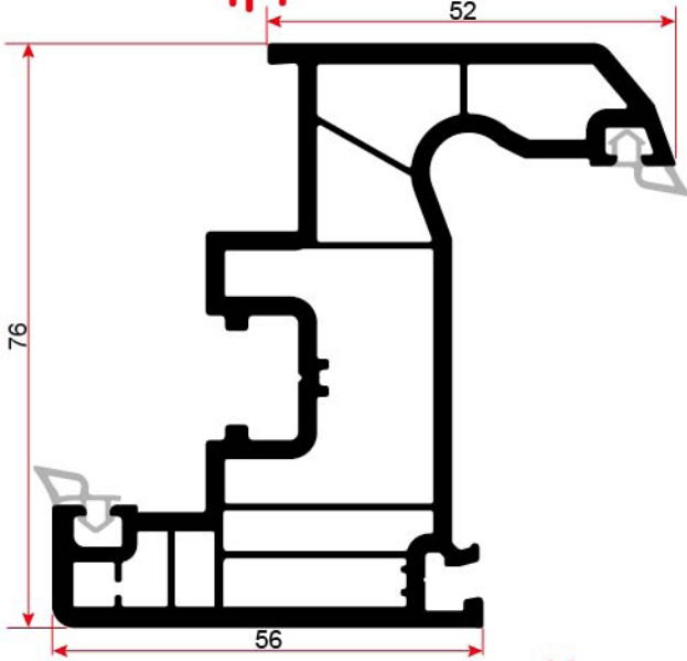
2205 PERVAZLI KASA PROFİLİ FRAME PROFILE WITH SILL
