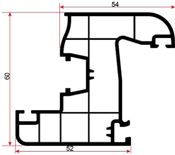
6005 PERVAZLI KASA PROFİLİ FRAME PROFILE WITH SILL
